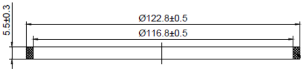
CORRECT GASKET
